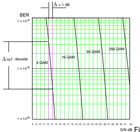
g. 2 BER in the range of 10^{-4} to 10^{-6} as a function of S/N in QAM
