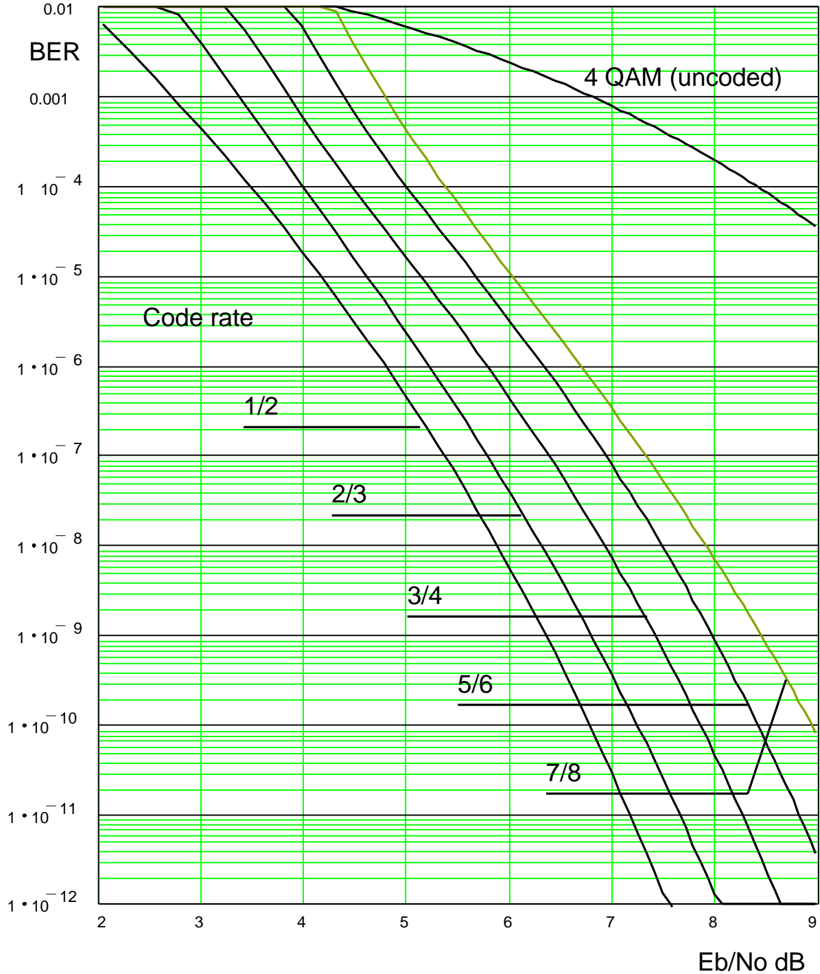
Fig. 13 BER as a function of Eb/No
