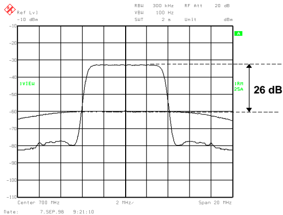
Fig. 9 PRBS useful signal and noise spectra with 10 dB/div
