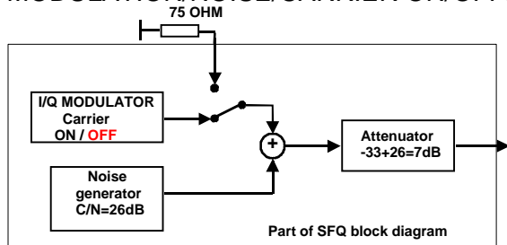
Fig. 8 CODER switched off by firmware and noise path in SFQ
