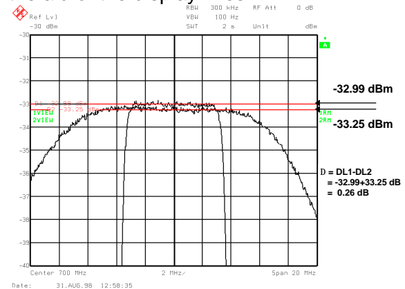
Fig. 9 Measurement of deviation from selected C/N value
