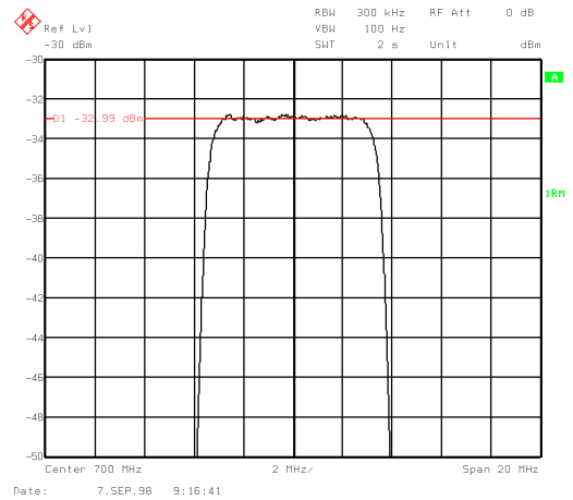
Fig. 6b PRBS spectrum: level marked with display line, 1 dB/div for highest precision
